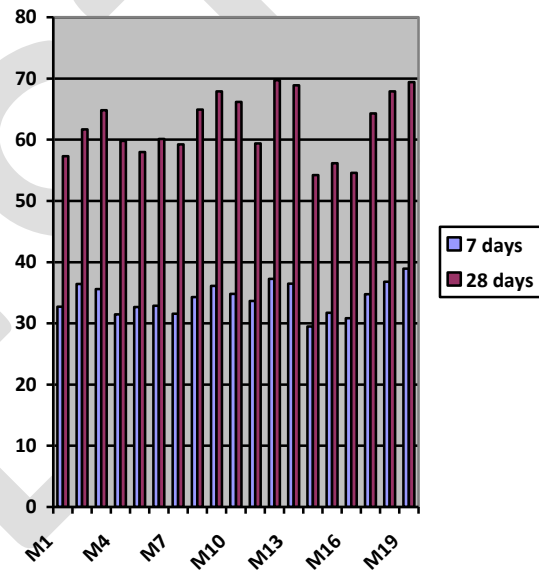
Figure 1. Compression test Results
